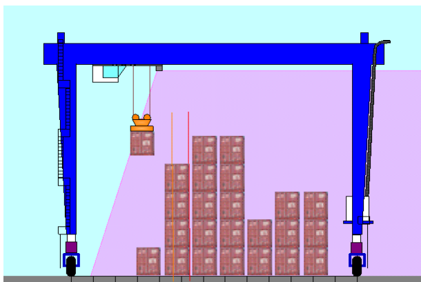
Figure 3 - Maxview Smart Move™ system.
